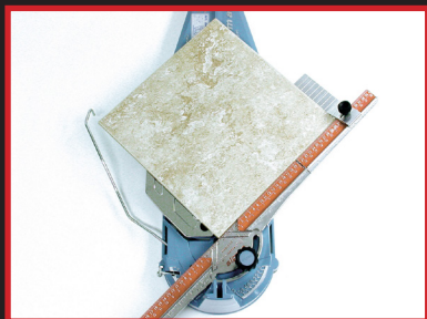
Rotate the guide to cut on a 45°
