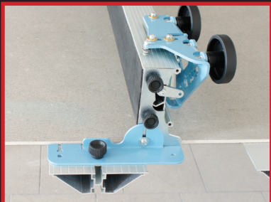
Shown using Kera-Cut Mounting Brackets (38F5)
