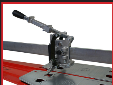
11 ball bearings for smoothness & accuracy
