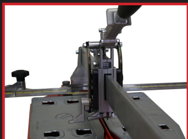
Single bar design for accuracy & strength
