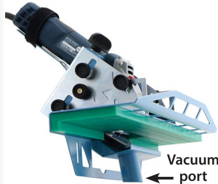
Setup for miter * Grinder not included
